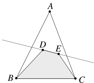
FIGURE 11.9. Finding a convex quadrilateral.
