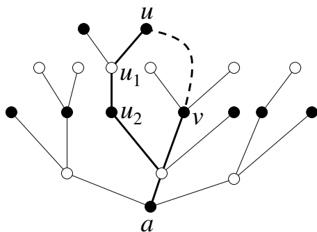
FIGURE 13.5. Bad 2-coloring yields an odd cycle.
