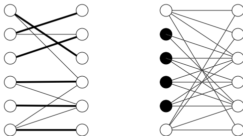
FIGURE 15.1. A bipartite graph with a perfect matching and one without
