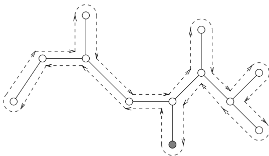
FIGURE 8.6. Walking around a tree.
