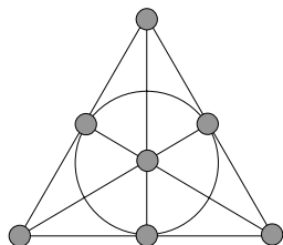
FIGURE 14.1. The Fano plane.
